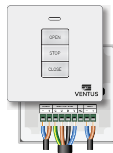
MR536 1 Channel Controller
