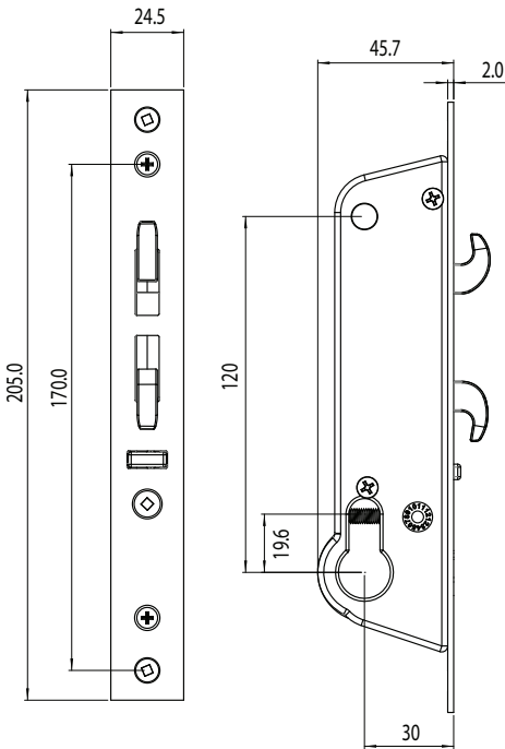
Lockbody
